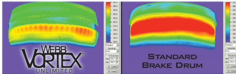
These photos taken from an infra-red camera mounted on the Webb Link dyno show a Webb Vortex® Unlimited drum next to a standard drum at precisely the same moment during braking. Compare the heat (red color) and you can actually see that Webb Vortex® Unlimited brake drums run significantly cooler.
